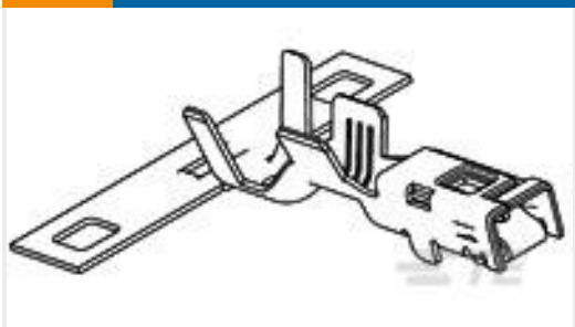
TE 产品编号1326032-5 2.8MM RECP,SEAL,14AWG
