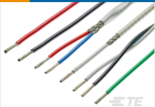
TE 产品编号306428-002 44AM1141-24-0/2/5/9-9
