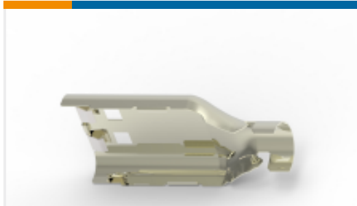
TE 产品编号1-2103157-2 SHIELD, PLUG, SIZE 2, Ag, HVA280
