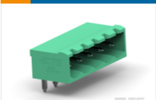
TE 产品编号1-2350513-0 10POS TB HDR 90 DEG, PITCH 5.0 &TL 4.5mm
