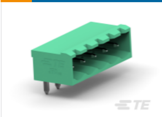
TE 产品编号1-2350513-0 10POS TB HDR 90 DEG, PITCH 5.0 &TL 4.5mm
