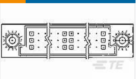
TE 产品编号5533061-5 ASSY,PIN,VERTICAL,HDI,LEAD-FRE
