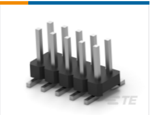
TE 产品编号2842142-5 10P,2MM,BRK HDR,DRV,T,SMD,0.1AU, TR W/CAP
