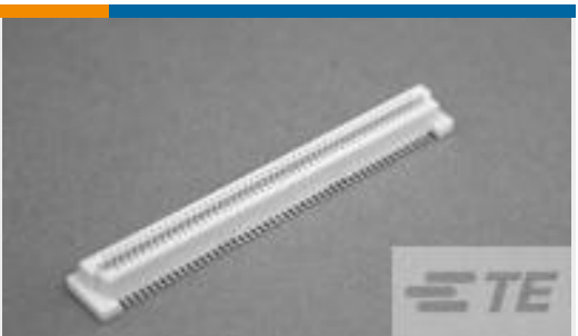
TE 产品编号2-1735482-2 0.8FH,R17H.5,060,30/Sn,TR,SC
