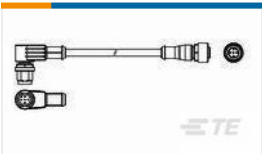
TE 产品编号2273120-3 M12 angled plug to M12 strgt socket AA
