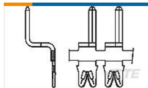
TE 产品编号1601070-2 131-137-014= TAB, 059X032, STDSMZ
