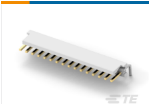
TE 产品编号 4-644761-6 16P MTA156 HDR ASSY R/A F/L LF
