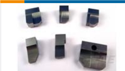
TE 产品编号3-1333200-8 ANVIL, COMBINATION .033 - .046
