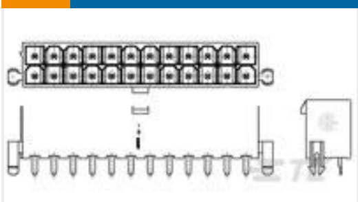
TE 产品编号2-2029059-4 24P VAL-U-LOK VRTHDR W/PGS GW
