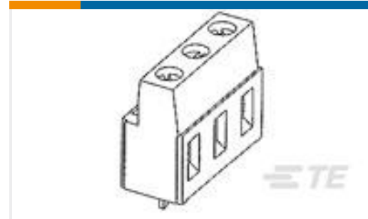
TE 产品编号282861-3 TERMI-BLOK PCB MOUNT 90 3P.7
