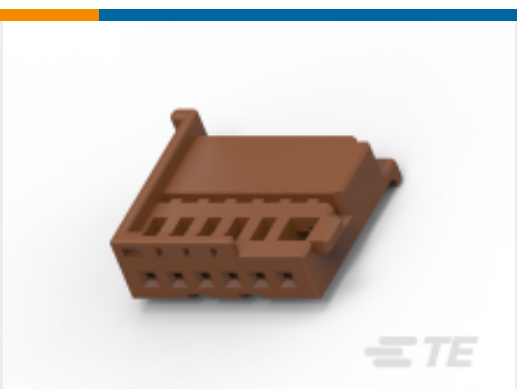
TE 产品编号1-969489-2 6POS MOS REC COD A
