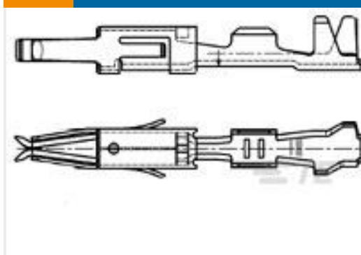
TE 产品编号1241844-2 MT2 A REC 1.6 Contact SRC Sn
