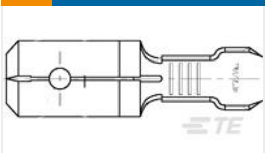
TE 产品编号60006-2 FASTON 250 TAB 18-14 AWG .031 TPBR
