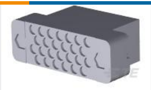
TE 产品编号200512-3 FEMALE BLOCK 26 PL.
