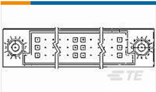
TE 产品编号532433-4 HDI PIN ASSY 3 ROW 105 POS
