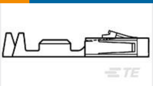
TE 产品编号1-104481-2 SHORT POINT RECP CONT LP
