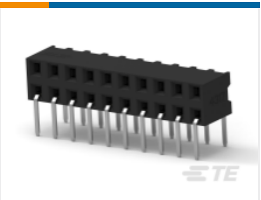
TE 产品编号2-2314926-0 20P,2MM,B-B,REC,DRHZ,2.8,0.76AU,TR
