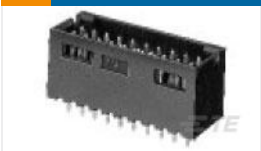
TE 产品编号1-103168-8 40 MODII HDR DRST SHRD .100CL
