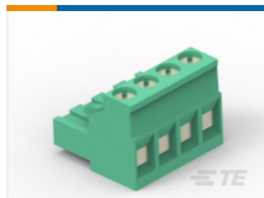
TE 产品编号 796634-9 9 POS 5.08MM R/A PLUG, TRM BLK
