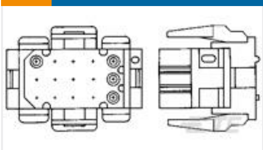
TE 产品编号1-640525-0 24P MR II PLUG HSG V0 RED
