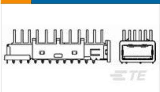
TE 产品编号2170125-1 XFP KIT W/CAGE, CLIP, 10mm HEAT SINK
