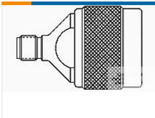
TE 产品编号1057403-1 ADAPTER, N PLUG TO SMA JACK
