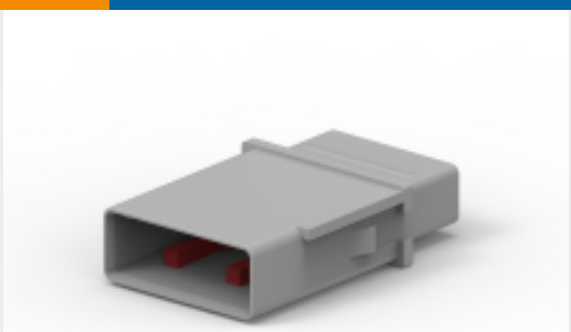
TE 产品编号284944-2 12 POS. MALE MODULE ASSEMBLY
