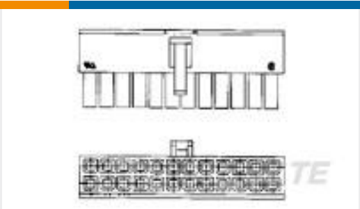
TE 产品编号2398990001 HT-SCE-1-2.0-0
