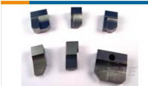
TE 产品编号 1333211-2 ANVIL, COMBINATION .150-.300
