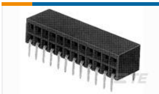
TE 产品编号2-102278-4 MOD II DBL ROW RECP ASSY
