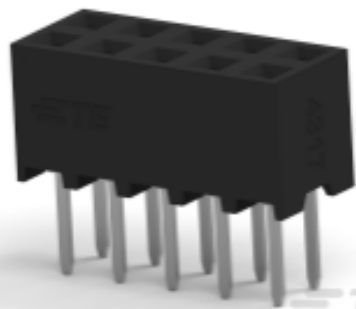
TE 产品编号1-2314822-0 10P,2MM,B-B,REC,DRV,T,2.7,0.76AU,TB
