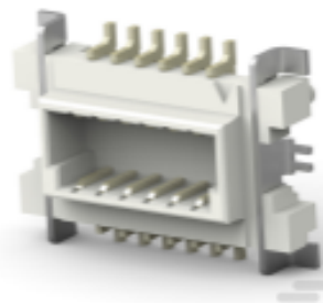
TE 产品编号1-179397-2 ON TAPING(EMBOSS) 0.8FS 3.0MM
