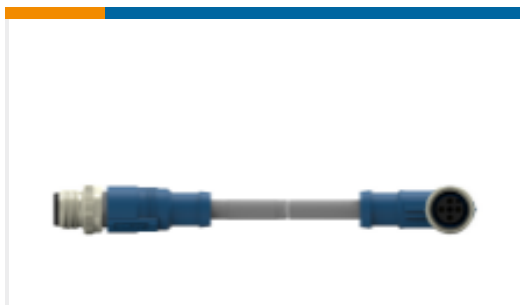
TE 产品编号T4162124004-005 RPC-M12-4MS-5.0SH-M12-4FR-PUR
