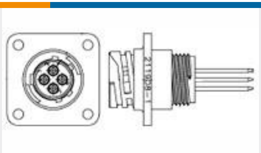
TE 产品编号1-788130-1 CPC RCPT,PSTD,SZ 11-4 LF
