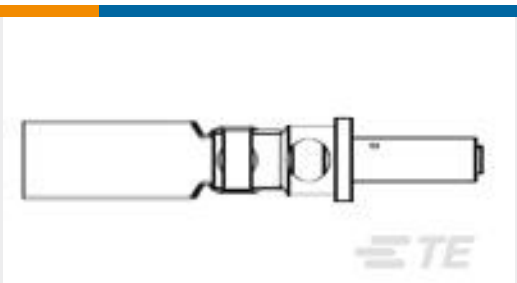
TE 产品编号YDTS20T25-35PAV001 RECP ASSY
