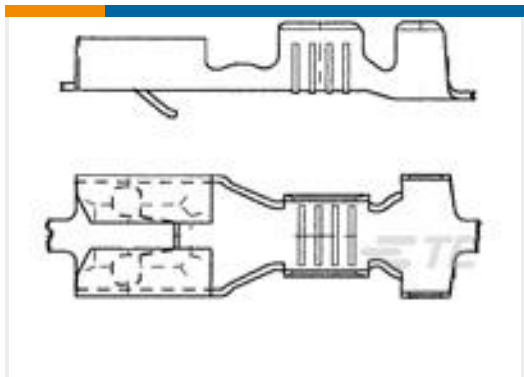
TE 产品编号282180-1 FF 187 REC 0.5-1.5MM2 TPBR
