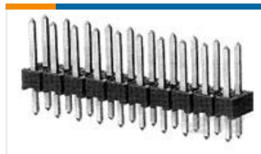
TE 产品编号1-826658-0 2X10 POS AMPMODU II PIN HEADER
