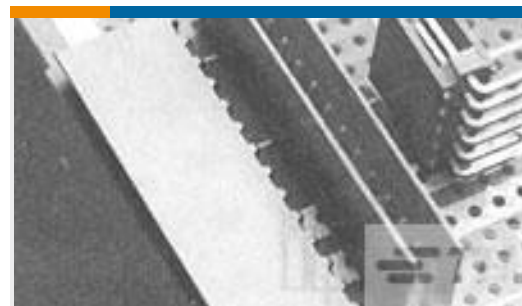
TE 产品编号281695-7 HEADER HE14 STRAIGHT 7 P
