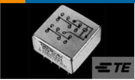
TE 产品编号2-1617076-5 3SBH1230A2 = M39016/53-011M
