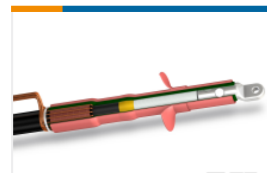
TE 产品编号CF6304-015 POLT-42E/1XI-ML-5-13
