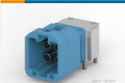
TE 产品编号2304168-3 4POS MATE-AX, HDR ASSY,90 DEG, COD C
