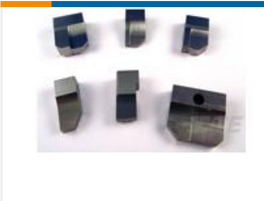
TE 产品编号2-1633928-1 ANVIL COMBINATION
