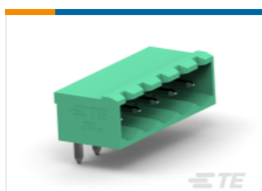
TE 产品编号1-2350513-5 15POS TB HDR 90 DEG, PITCH 5.0 & TL 4.5mm
