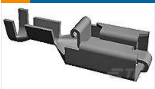
TE 产品编号154717-1 PL 250 REC TERMINAL 13-11 AWG BR
