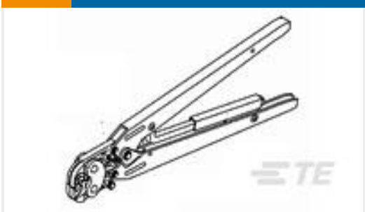
TE 产品编号755342-1 DAHT POS LOCK REC CONT 20-14 ASSY
