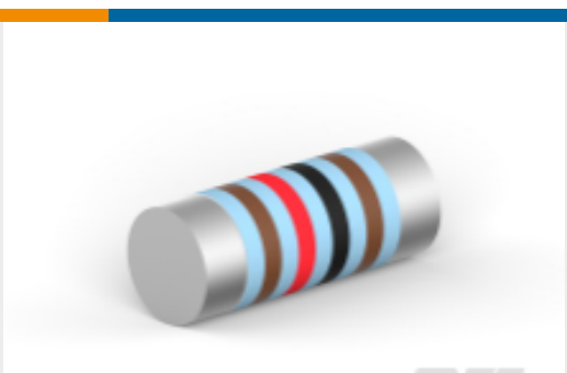
TE 产品编号1-1879283-6 MELF SMA 2K74 0.1% 25PPM 0.25W
