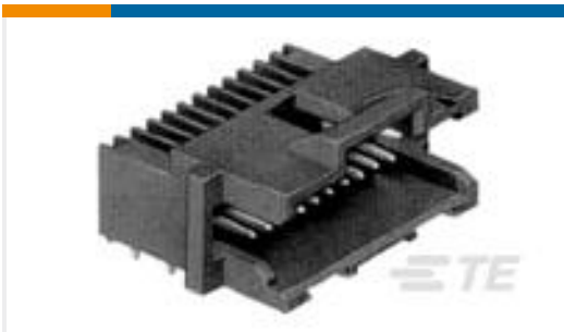
TE 产品编号1-104477-2 10 SYS50 HDR DRRA W/.145 SOLDE
