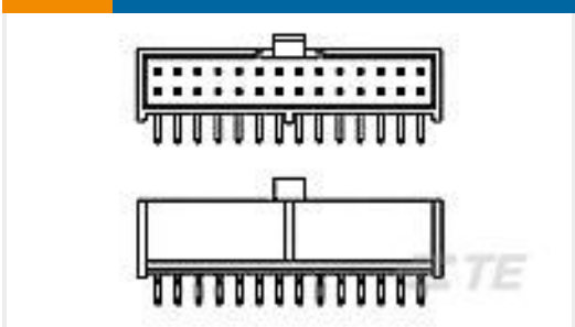
TE 产品编号1888292-9 FPH-1602G=FLXPAC HDR P 16 RA LF
