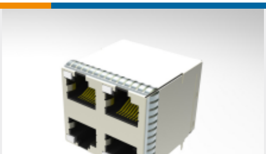
TE 产品编号2303402-1 STK MJ ASSY,8POS,2X2,CAT5E
