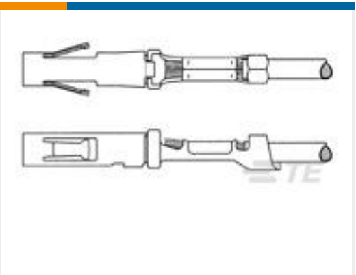
TE 产品编号164153-6 CONTACT, SOCKET, CRIMP, TYPE XI
