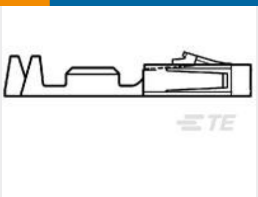
TE 产品编号1-104480-4 SHORT POINT RECP CONT LP
