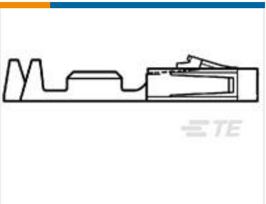
TE 产品编号1-104480-2 SHORT POINT CONT 15 DPLX STMPD LF
